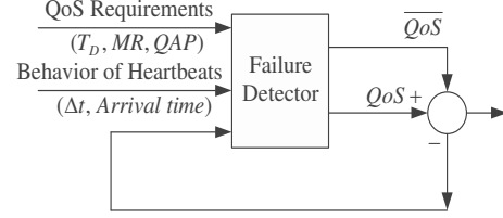
Fig. 4. Feedback architecture in self-tuning failure detector with the target \overline{MR} and \overline{T_D} .
