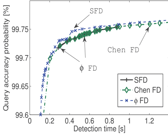
Fig. 7. Query accuracy probability vs. detection time in a WAN.
