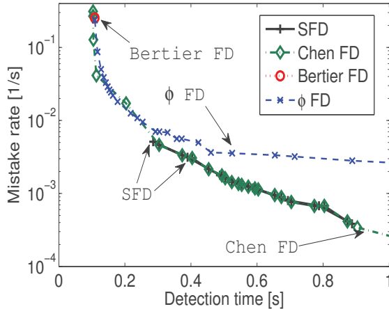
Fig. 6. Mistake rate vs. detection time in a WAN.
