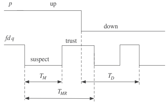
Fig. 3. Basic Metrics for the QoS evaluation of an FD [28].
