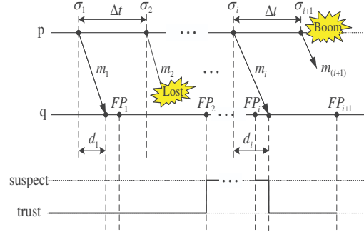
Fig. 2. Basic heartbeat failure detection model.
